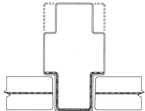
Mullion
