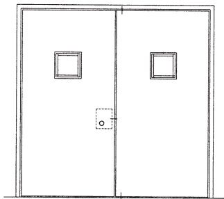
Pair of Doors (No Mullion) Door Mounted Lock 2 Singles Welded Mullion Between Doors Door Mounted Lock
