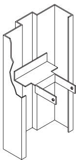
FIGURE 5A WOOD STUD ANCHOR Z ANCHOR
